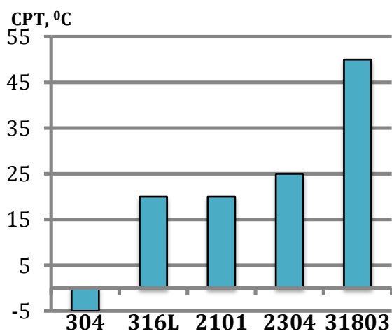
Critical Pitting Corrosion: (As per ASTM G150)
