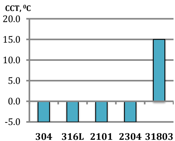
Critical Crevice Corrosion (As per ASTM G48 Method F):
