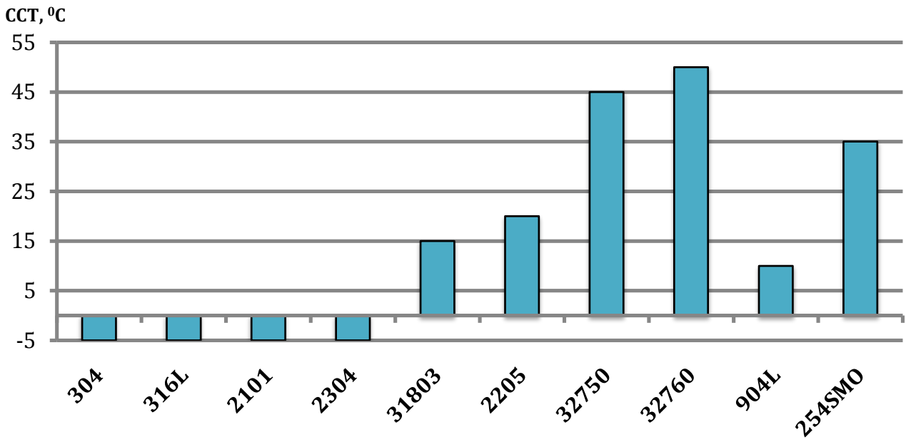
Critical Crevice Corrosion: (As per ASTM G48 Method F)
